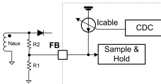
Fig.5 CDC block
